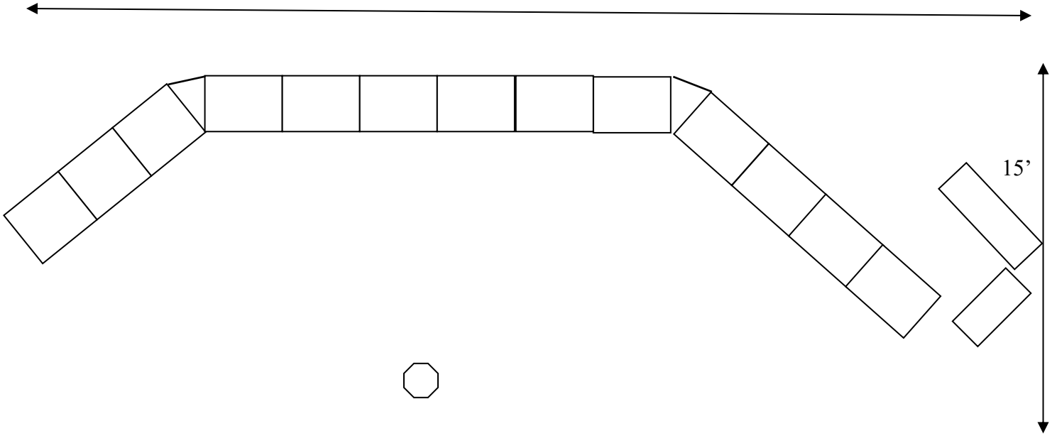
Wedged U Layout – 5 Octaves + Bass Chimes
